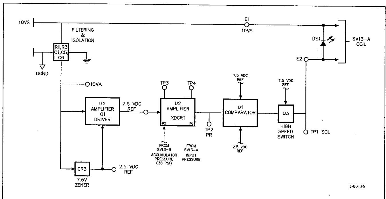
Figure 7-14. I/O (Input/Output) PCA Block Diagram
