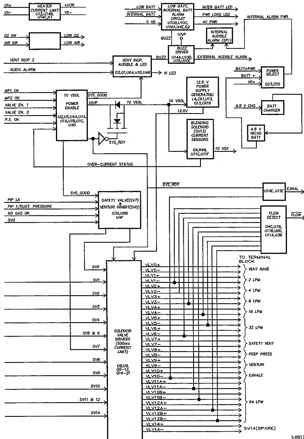
Figure 7-20. Alarm Driver PCA (current limiting) Block Diagram
