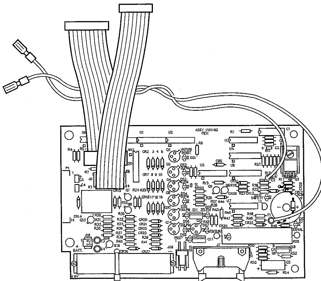
Figure 7-15. Alarm Driver PCA
