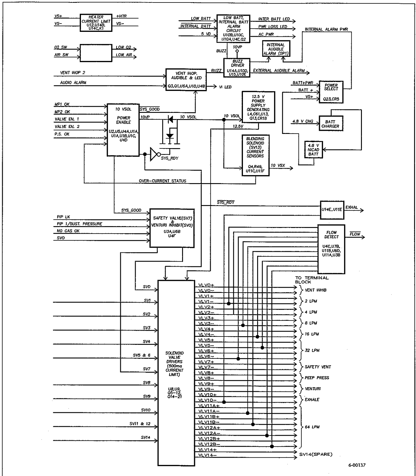
Figure 7-16. Alarm Driver PCA Block Diagram
